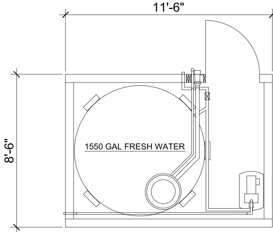
8'-6"X11'-6" FRESH WATER FLOOR PLAN
