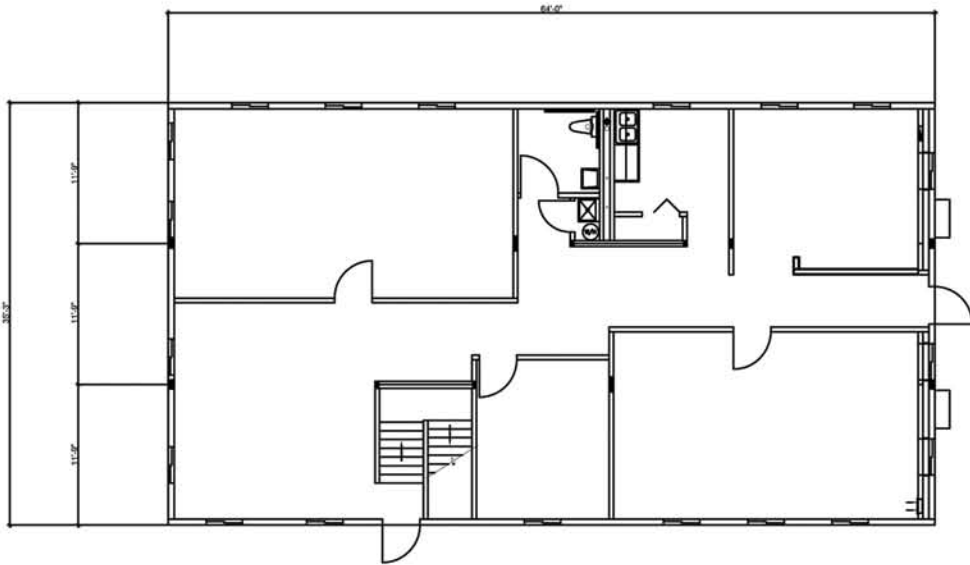
1st FLOOR
